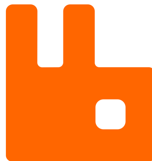
RabbitMQ
